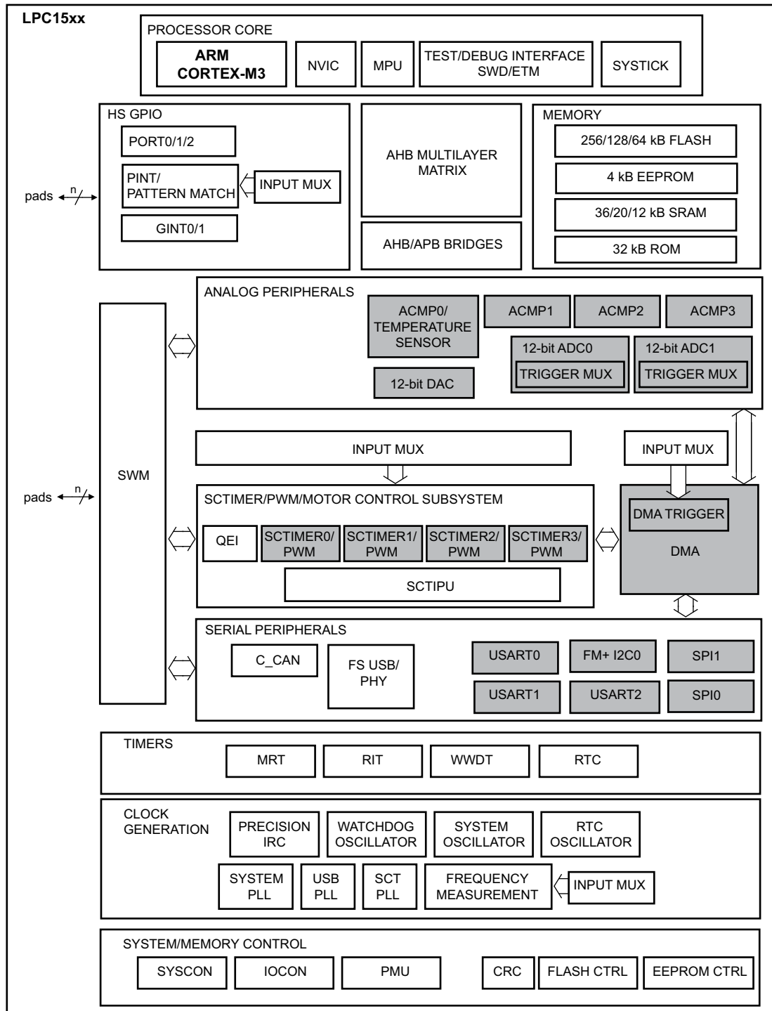
Fig 1. Block diagram
