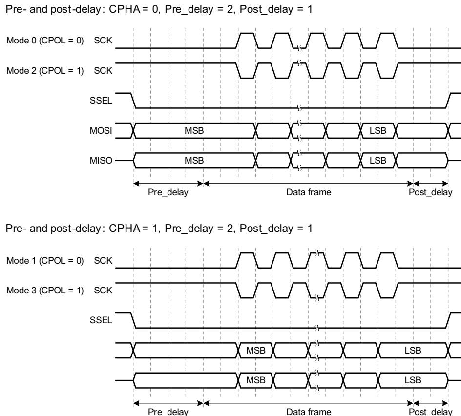
Fig 70. Pre_delay and Post_delay
