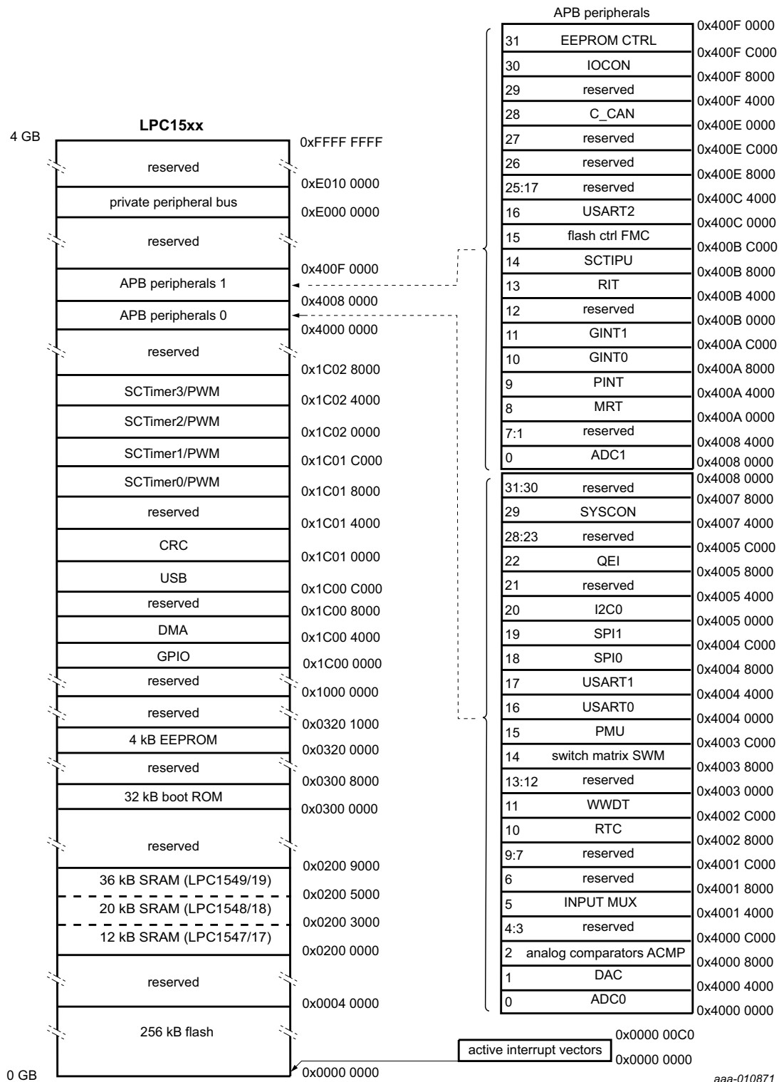
Fig 1. Memory mapping
