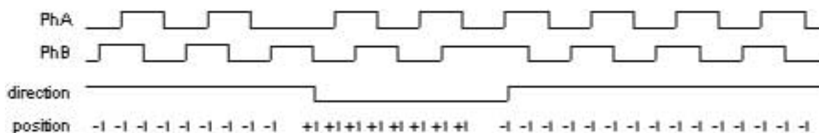
Fig 57. Quadrature Encoder basic operation
