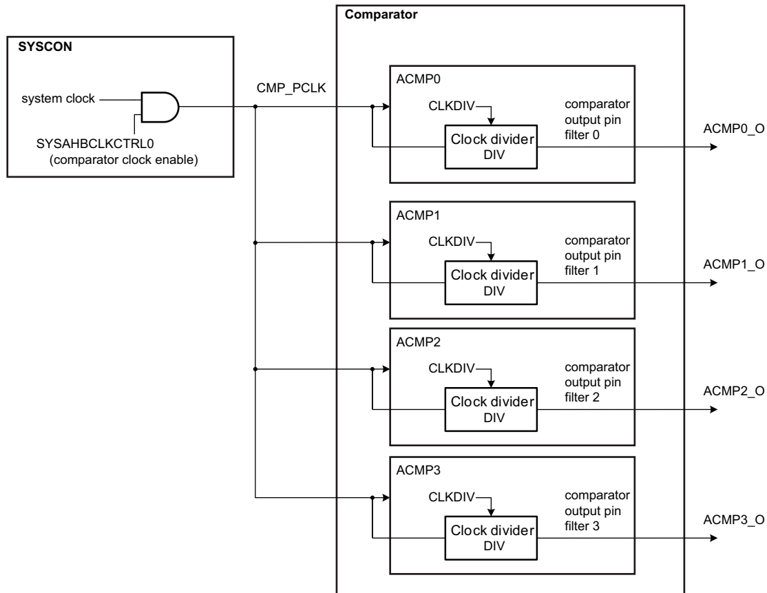
Fig 87. Comparator clocking
